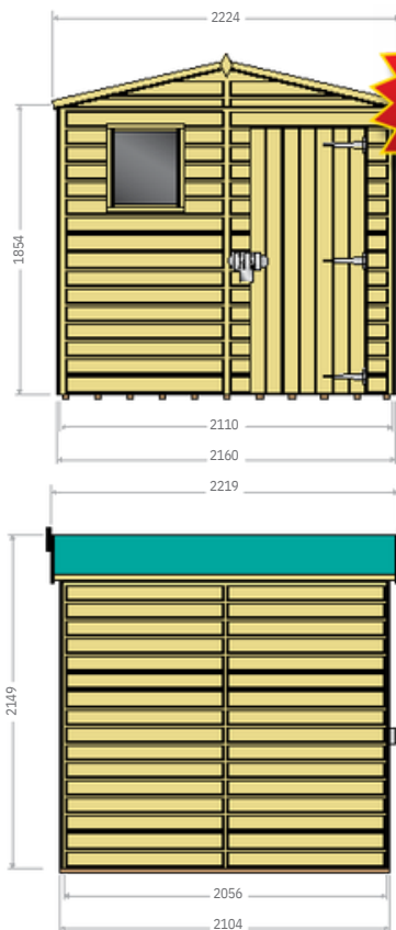
Modular Shiplap and Overlap shed
